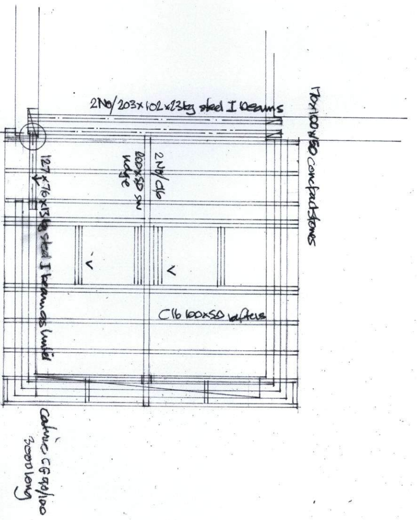
ROOF STRUCTURE PLAN
